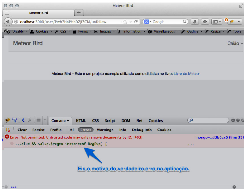
Figura . : Erro: Not permitted. Untrusted code may only remove documents by ID.
